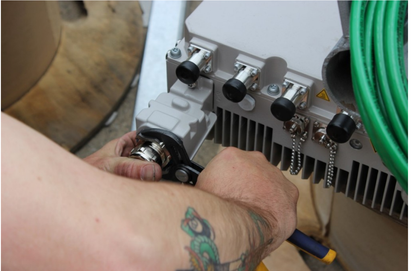
Alcatel-Lucent Remote Radio Head - 3JR41102ABA RRH8X20-25-FEU_8[/caption]
